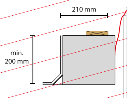
Concrete with wooden batten
